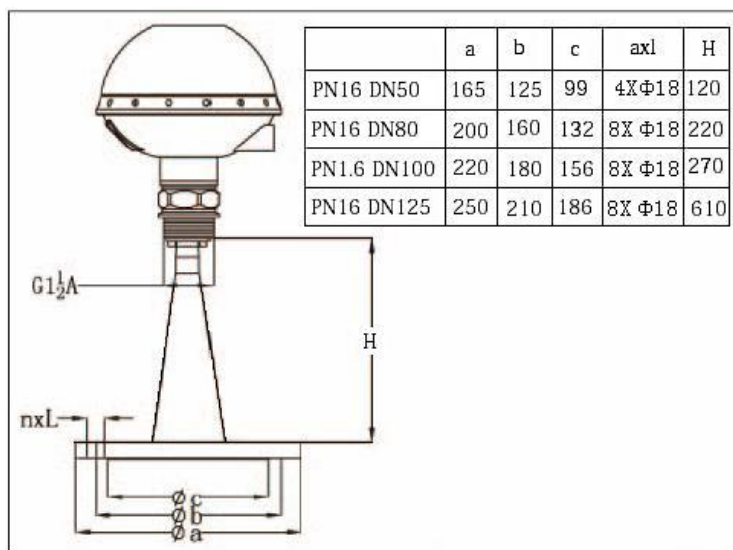
Flange Installation
