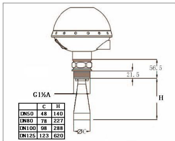
Thread Connection
