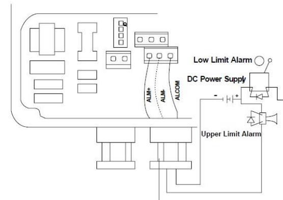
Connection of Alarm Output
