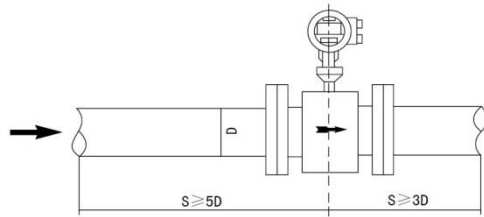
Picture a Horizontal pipe Length Requirements to front and back straight pipe part
