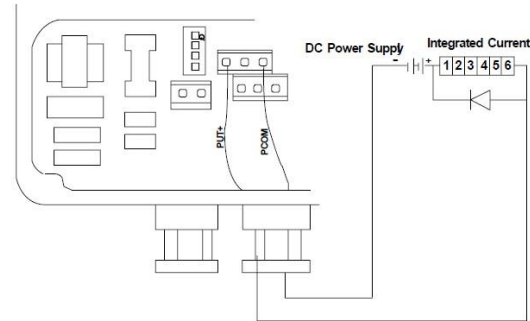
Connection of Electromagnet Counter
