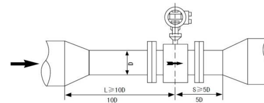
Picture c Flaring pipe Length Requirements to front and back straight pipe part
