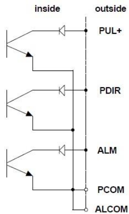
Connection of OC Gate
