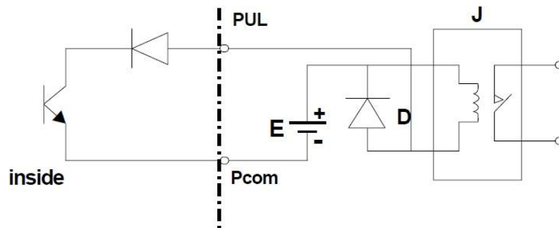
Digital Quantity Output Connecting Relay
