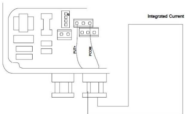
Connection of Electronic Counter
