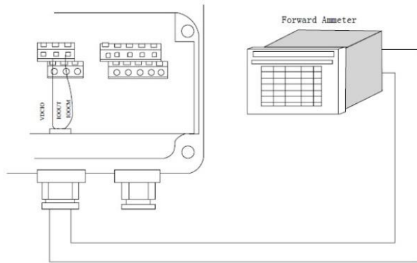
Current Output Diagram
