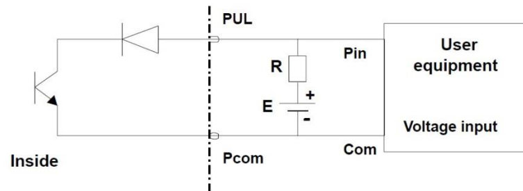
Connection of Digital Quantity Electrical Level Output
