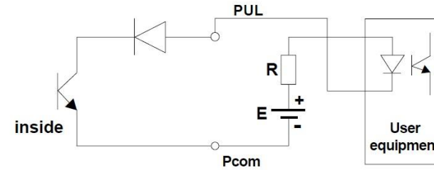
Digital Quantity Output Connecting Photoelectric Coupler
