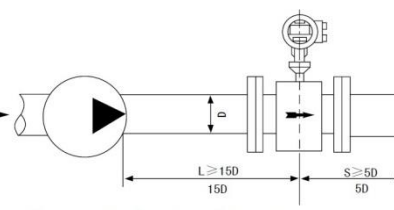
Picture f Backward position of mercury Length Requirements to front and back straight pipe part
