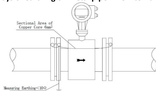
Mounting of Sensor in Metallic Pipeling (inner wall has no insulating layer)
