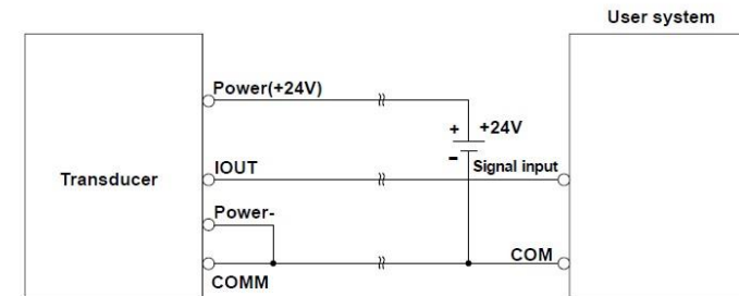
3-wire connection
