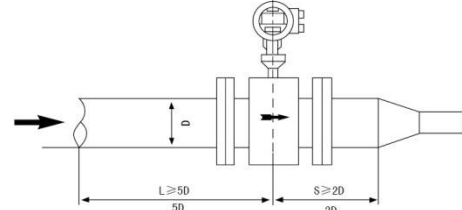
Picture e Shrinkage pipe Requirements to front and back straight pipe part
