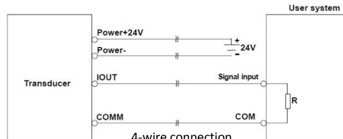
4-wire connection
