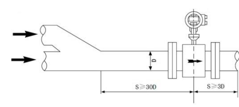
Picture g Mixed liquid Requirements to front and back straight pipe part
