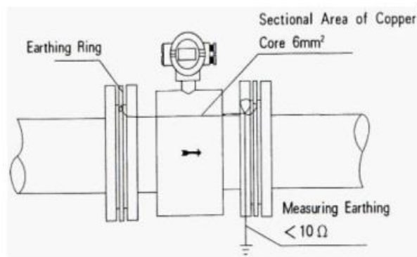
Mounting of sensor on plastic pipeline or pipeline with insulating layer or paint
