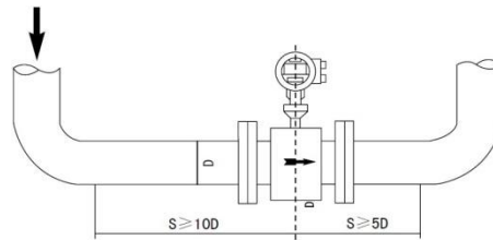
Picture b Bent pipe Length Requirements to front and back straight pipe part
