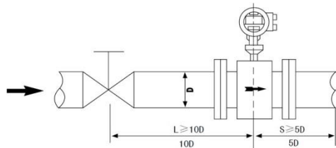
Picture d Backward position of valve Length Requirements to front and back straight pipe part
