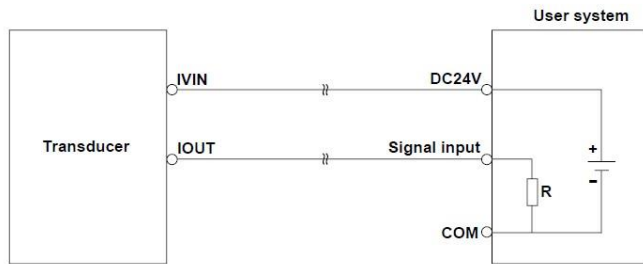
2-wire connection
