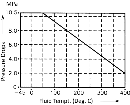
Fig. 2 GLAND PACKING PRESSURE-TEMPERATURE RATINGS
