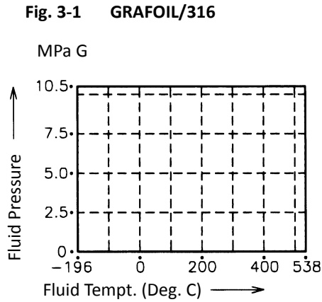
Fig. 3 GASKET PRESSURE-TEMPERATURE RATINGS
