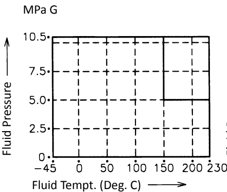
Fig. 2-2 TFE FIBER/TFE- ASBESTOS
